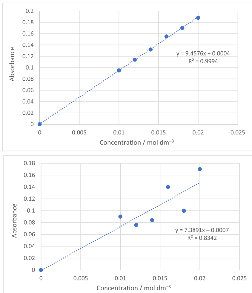
Best-fit lines for concentration vs absorbance data from two experiments
