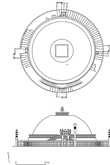
Plan and elevation
